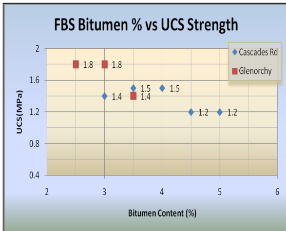
Figure 5: Bitumen % Vs UCS Strength
