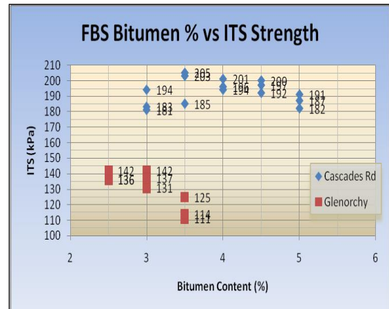
Figure 6: Bitumen % Vs ITS Strength
