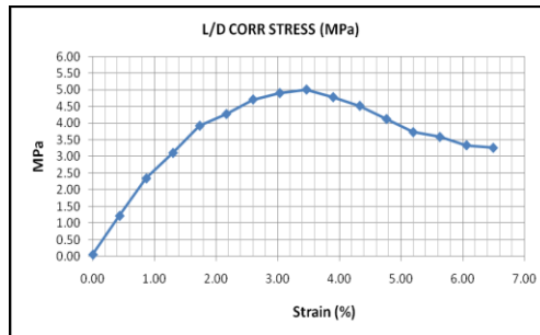
Figure 2: UCS Plot for FBS Dacite
