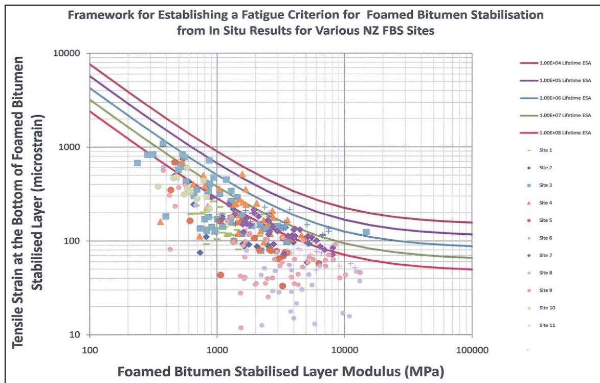
Figure 17: FWD Derived Basecourse Modulus vs Strain for New Zealand FBS sites.
