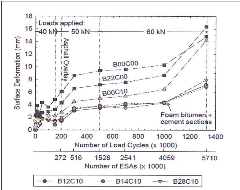
Figure 18: Rut Development Versus No. of Load Cycles for NZ CAPTIF Experiment
